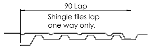
Figure 7.4 Lap Section
