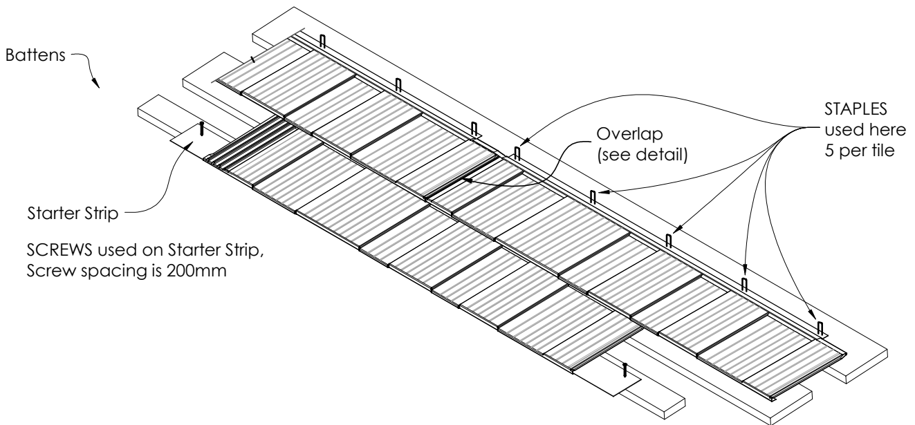
Figure 7.2 Fastening Detail
