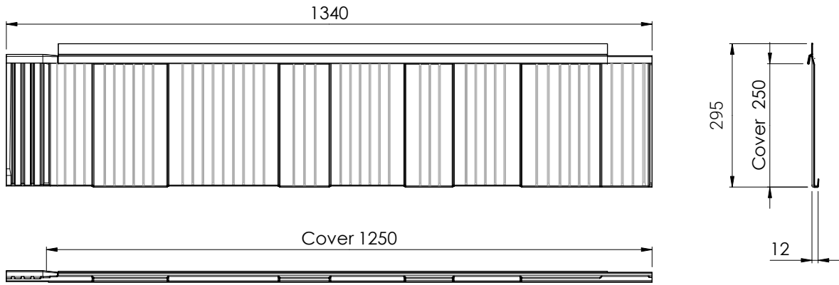
Figure 7.1 Tile Dimensions
