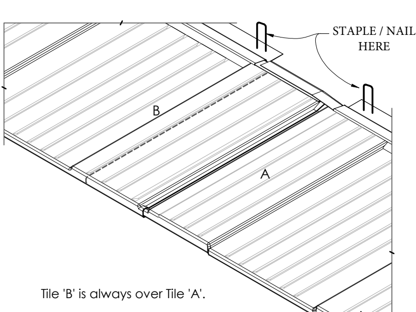
Figure 7.3 Overlap Detail
