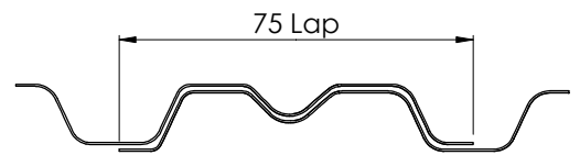
Figure 2.4 Lap Section
