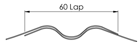
Figure 1.4 Lap Section
