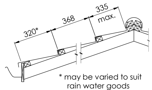
Figure 8.5 Batten Layout
