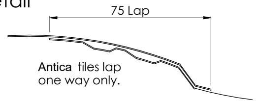
Figure 8.4 Lap Section
