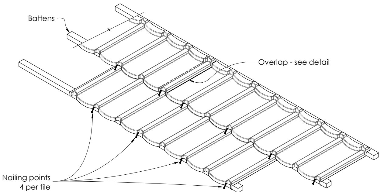
Figure 6.2 Nailing Detail
