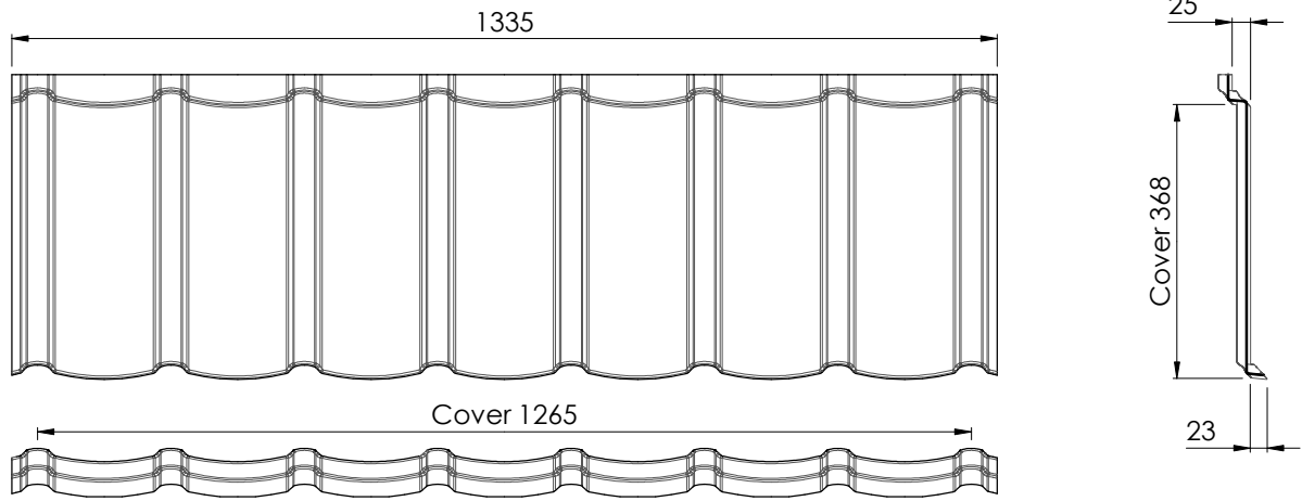
Figure 6.1 Tile Dimensions
