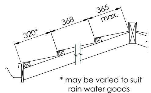
Figure 6.5 Batten Layout
