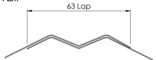
Figure 4.4 Lap Section
