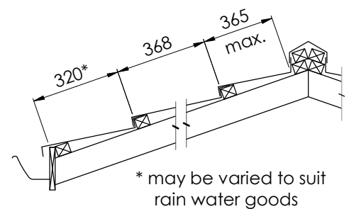
Figure 5.5 Batten Layout
