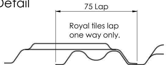
Figure 5.4 Lap Section
