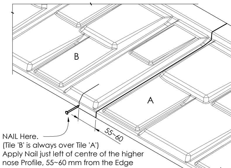
Figure 5.3 Overlap Detail
