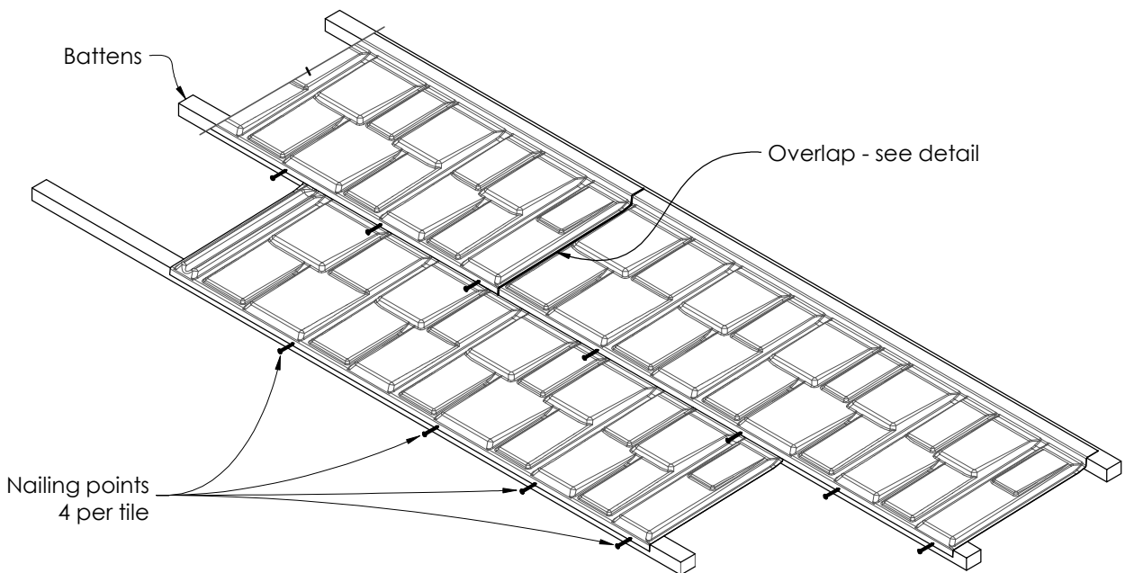
Figure 5.2 Nailing Detail
