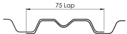
Figure 2.4 Lap Section
