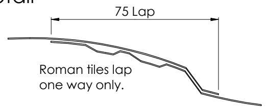
Figure 3.4 Lap Section
