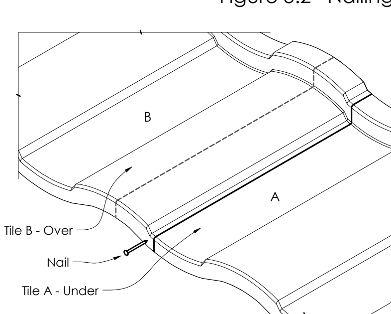
Figure 3.3 Overlap Detail
