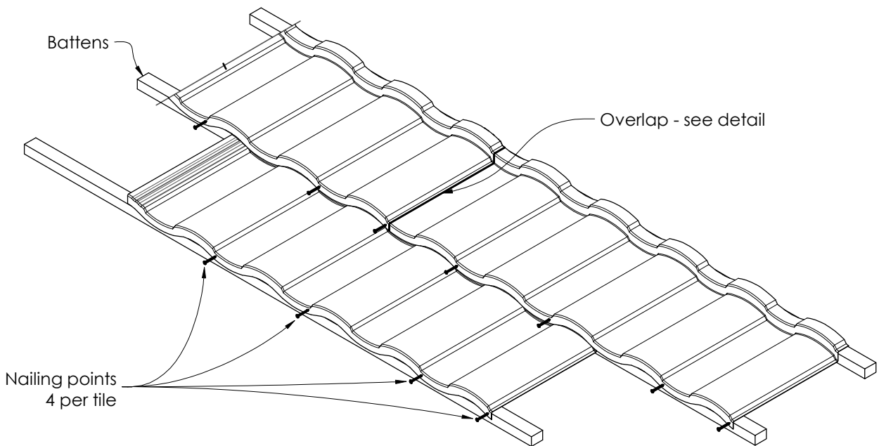
Figure 3.2 Nailing Detail
