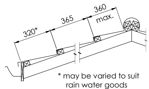
Figure 3.5 Batten Layout
