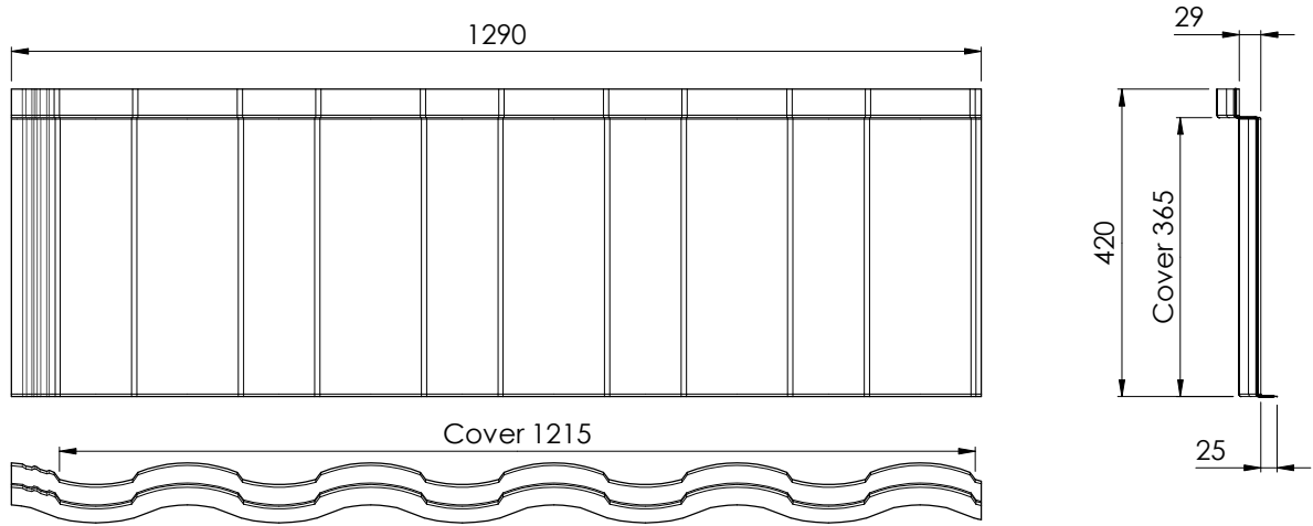
Figure 3.1 Tile Dimensions
